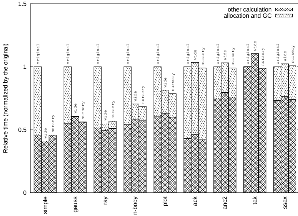
Figure 6: Time spent in allocation/GC and other calculation
